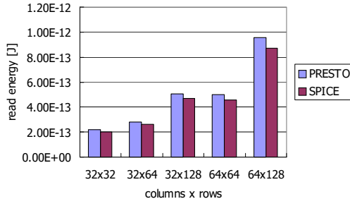
Fig. 6 SRAM read energy at 100nm process.
