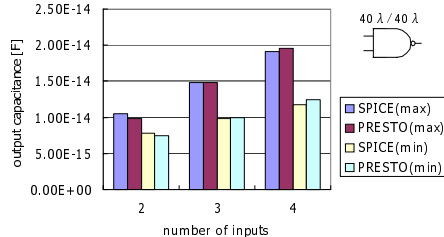
Fig. 5 Output capacitance of a NAND gate at 100nm process.
