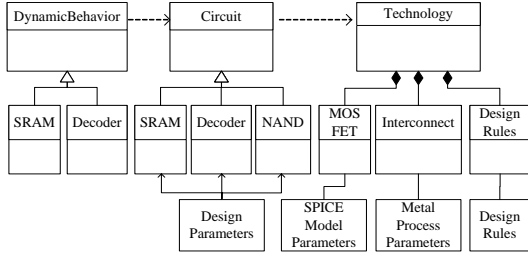
Fig. 2 Relationship between modeling layers.
