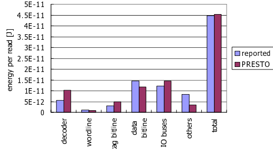
Fig. 7 Breakdown of energy consumption for 32-bit read accesses in base line cache.
