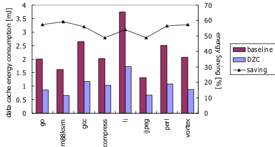
Fig. 8 Data cache energy consumption.
