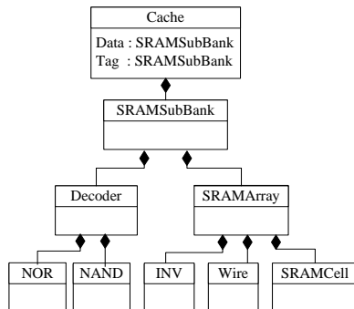
Fig. 3 Hierarchical implementation of cache class in the circuit layer.
