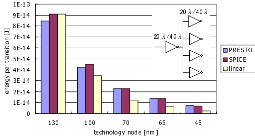
Fig. 4 Energy consumption of a FO4 inverter.
