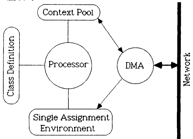
(図3) Processor Element
